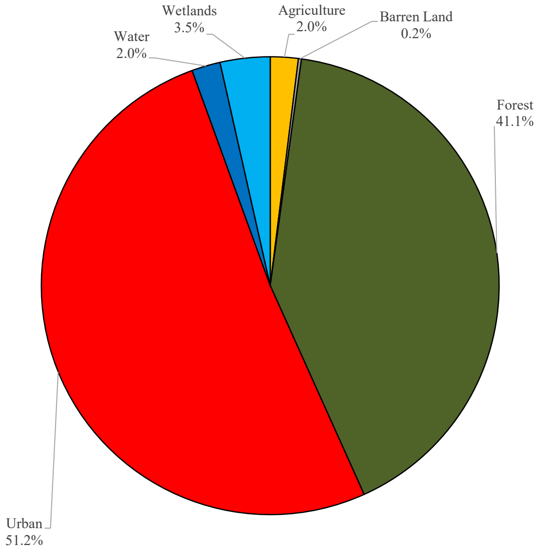
Figure 3: Pie chart illustrating the land use in High Bridge Borough
