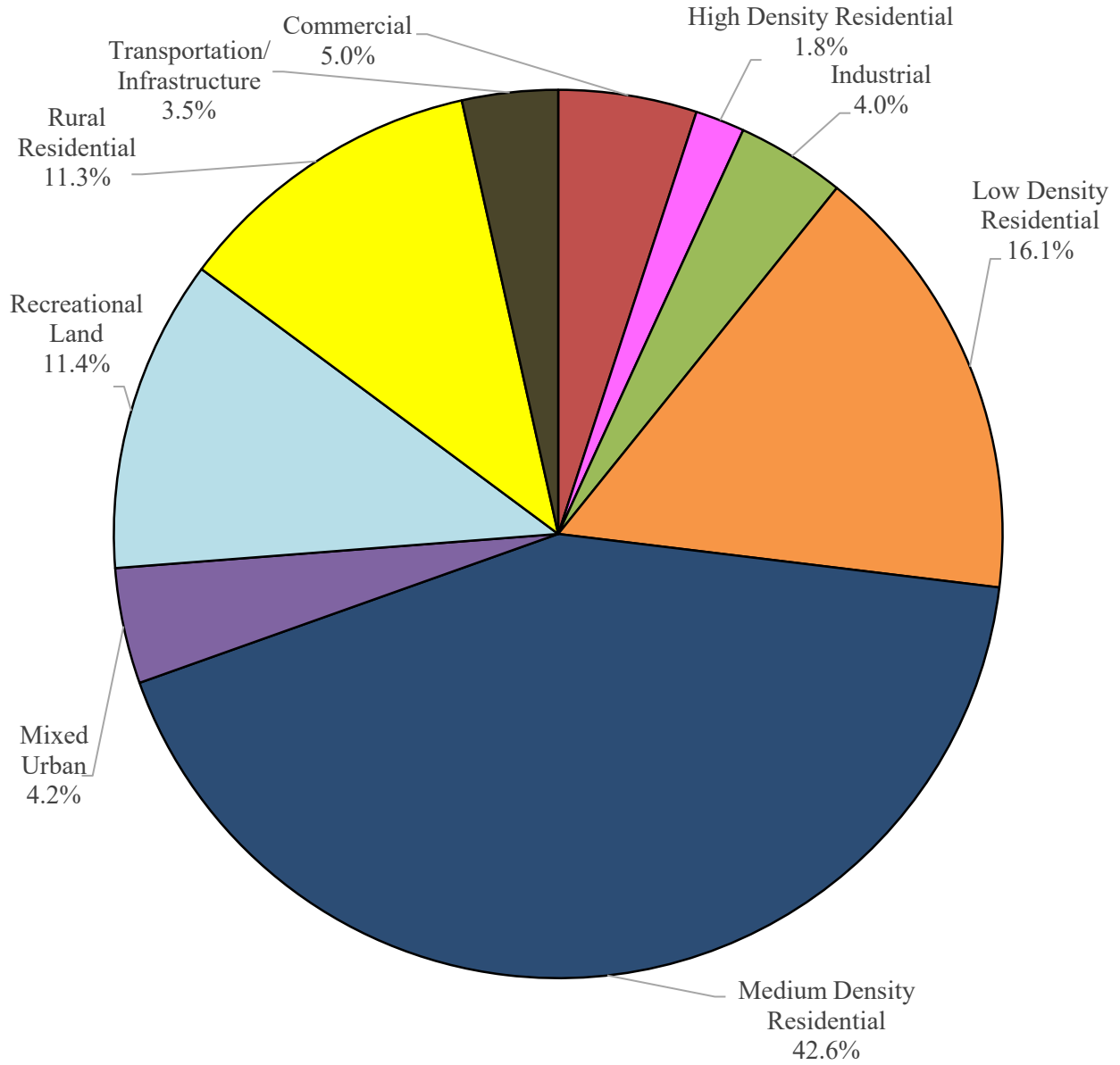
Figure 5: Pie chart illustrating the various types of urban land use in High Bridge Borough
